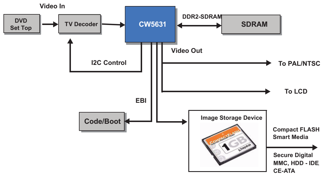
Figure 1-3 Digital Video Recorder (without LCD output)/Personal Media Player (with LCD output)
